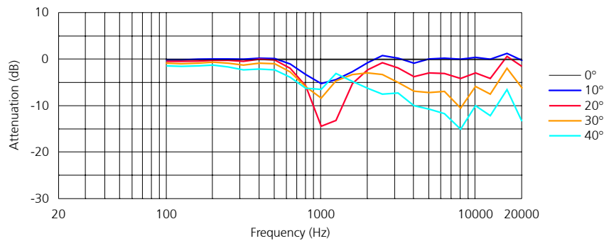
Vertikaler Frequenzgang ‚off axis up‘
