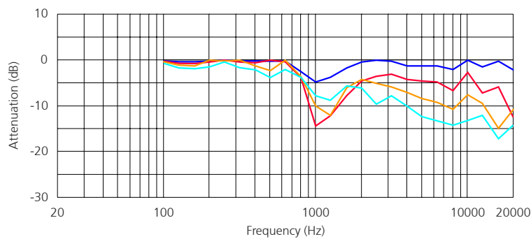
Vertikaler Frequenzgang ‚off axis up‘
